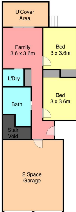
Lower Level
